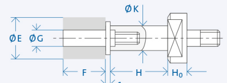
FIG. 3: FOR GRINDING WHEELS ON THREADED PIN (PL)*
